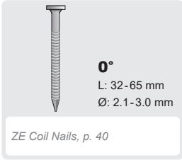
TJEP ZE-65 EXCELLENT
