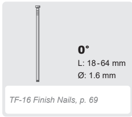
TJEP TF-16/64 GAS 3G
